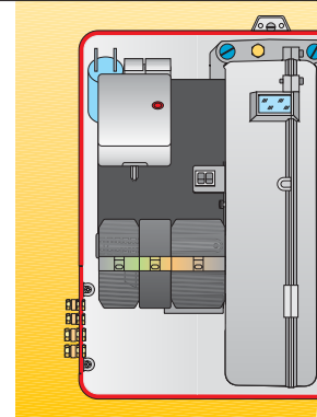
Example of plugs and sockets for electrical connections for the RS 28-38-50 models
